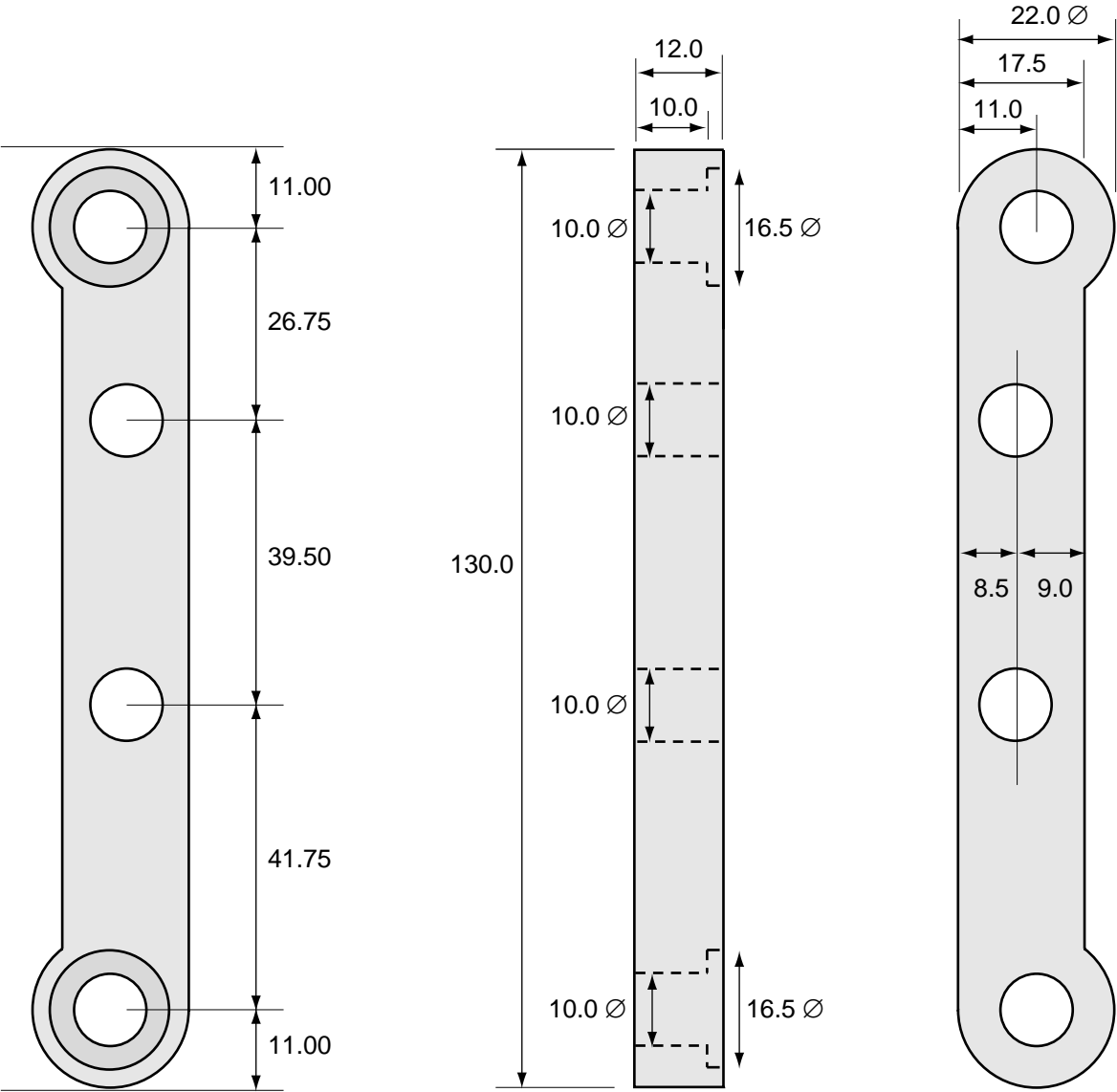
Adapter for right-hand fork leg
